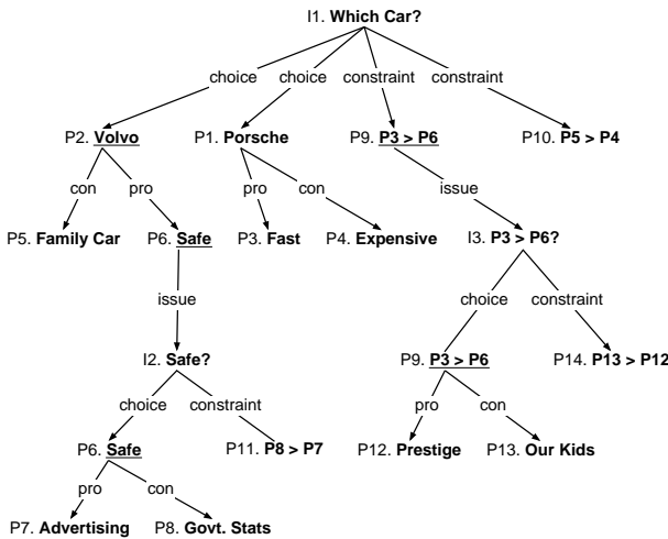
Figure 4: A Dialectical Graph
